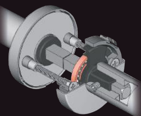
Pullbloc® 4.1 FS Panik
